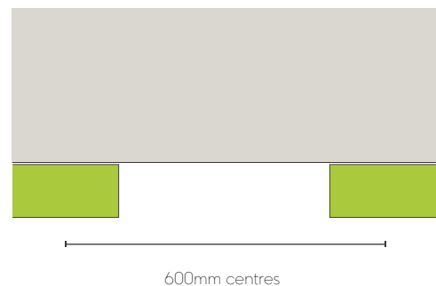
Fig 2 - Batten centres
